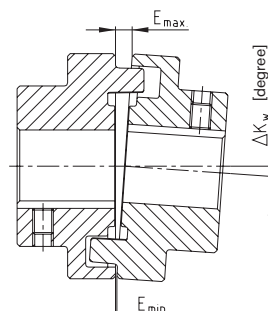
Angular displacement ΔK w
