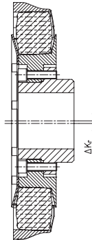
Radial displacement
