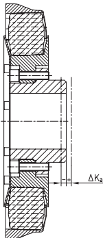
Axial displacement
