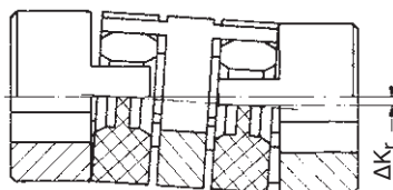
Radial displacement
