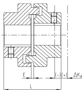
Axial displacement ΔK a
