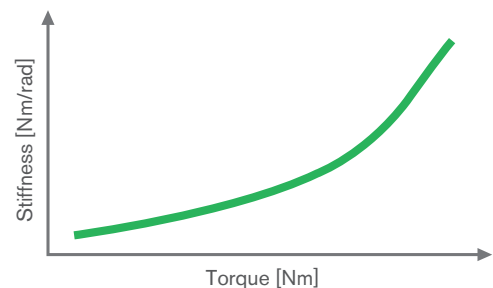
Stiffness characteristic (progressive)
