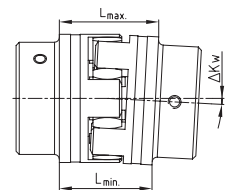
Angular displacement \Delta K_w [degree]
