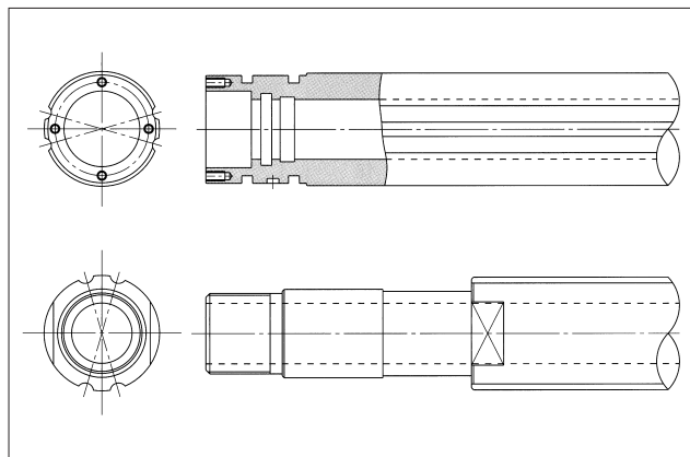
Figure B-22 Examples of Shaft End Machining
