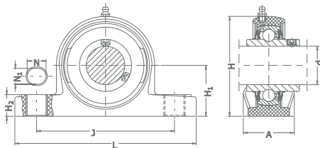
SYL housing (with zinc-coated bearing)
