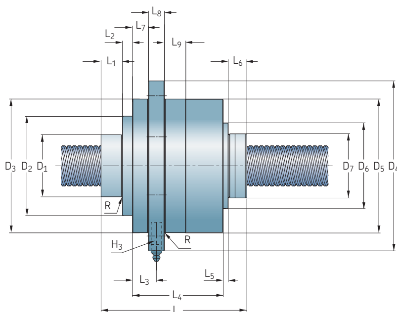
Screw Dimensions
