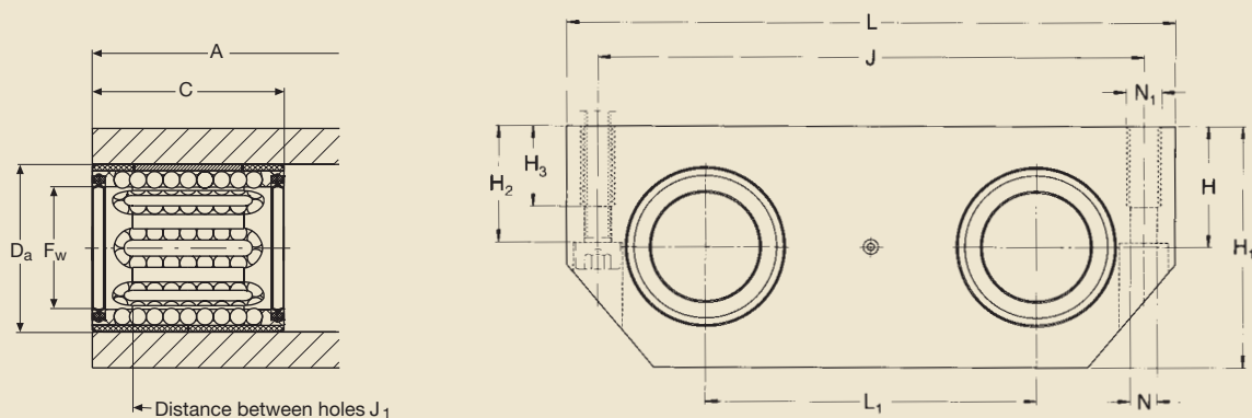
LQBR With double lip seals on the outside
