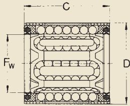
LBBR with double lip seals
